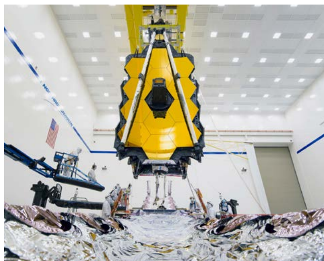
Integration team members use a crane to slowly lift Webb telescope into place above the Spacecraft Element. Engineers then connected the two halves of the telescope, completing a major milestone. Watch the team join the two halves. Photo credit: NASA/Chris Gunn
